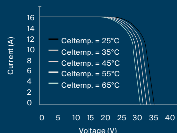
Current-Voltage (440W) (445W)
