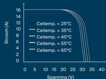
Stroom-Spanning (445W)
