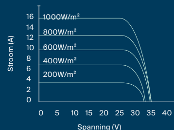
Vermogen-Spanning (445W)
