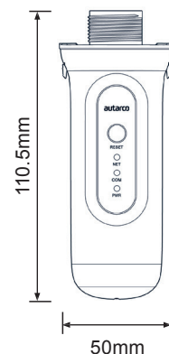
4G-STICK-D.U1 (4G + WiFi)
