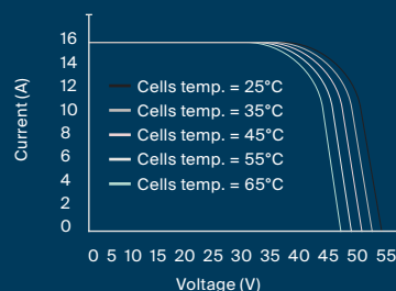
Current-Voltage (550W)
