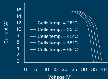
Current-Voltage (420W)
