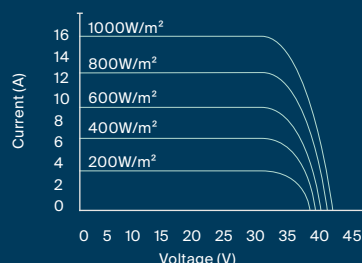
Current-Voltage (505W)
