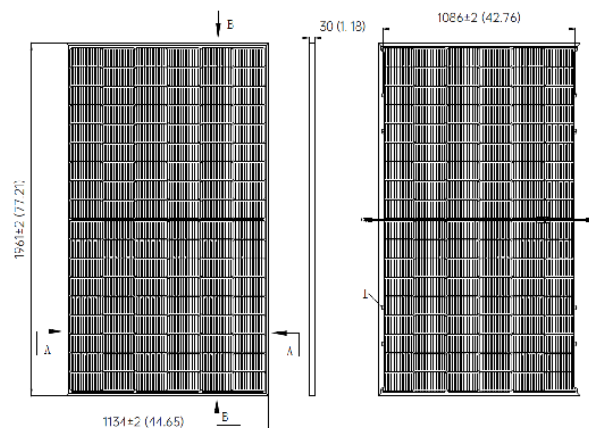
Solar panel
