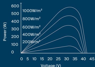
Power-Voltage (505W)
