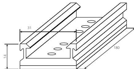
Bracket landscape mounting (mm)
