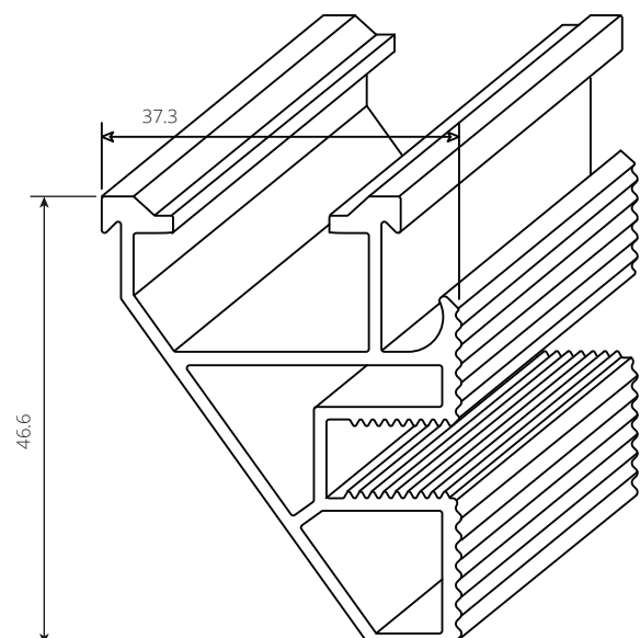
Rail section (mm)
