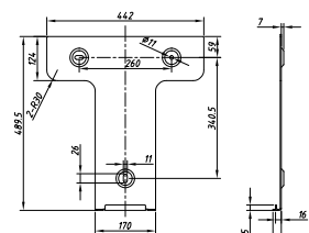
Bracket
