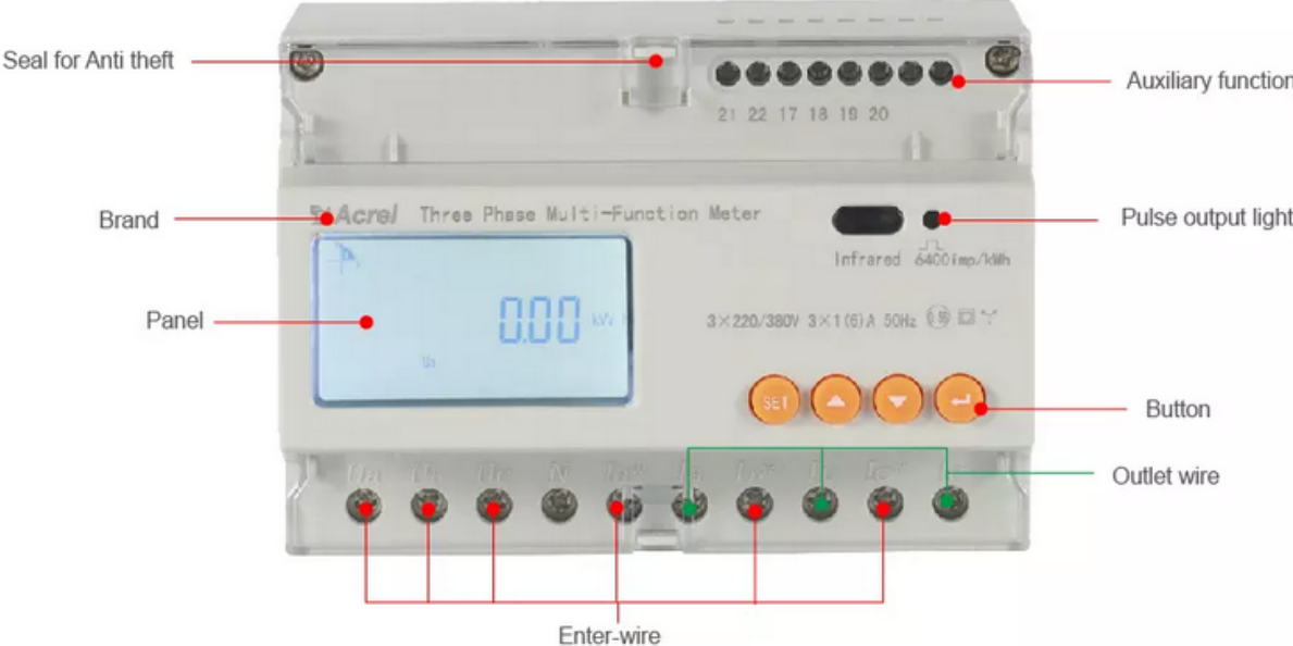
Figure 3.1: Front display
